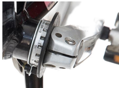
Foto 3.4 Hollowtech II
